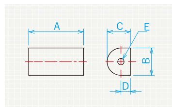
寸法図 Dimensional drawing
